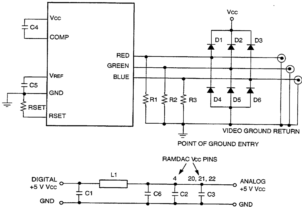
Figure 9. Typical Connection Diagram Using the Internal Voltage Reference
