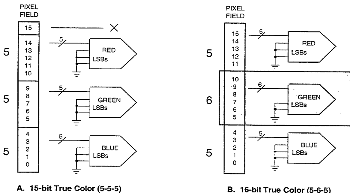
Figure 4. 15-/16-Bit Field Split for True-Color Modes
