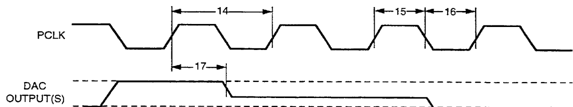
Figure 14. Video Timing
