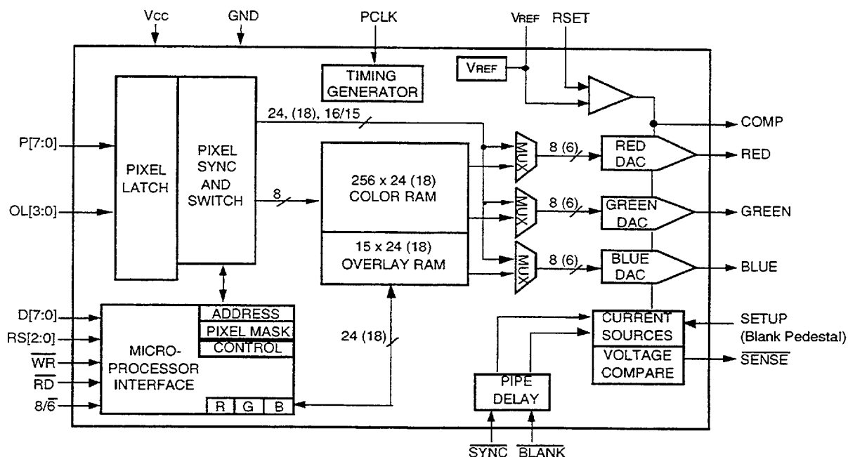
Figure 1. Block Diagram
