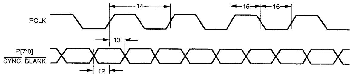
Figure 13. Pixel Timing
