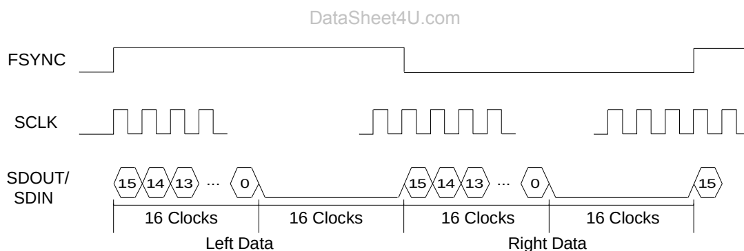
Figure 7. 64-bit mode (SF1,0 = 01)
