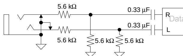
Figure 2. Line Inputs
