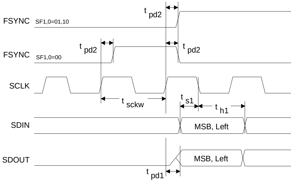
Serial Port Timing DataSheet4U.com
