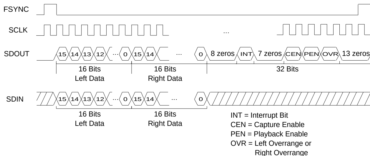
Figure 6. 64-bit enhanced mode (SF1,0 = 00)
