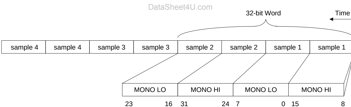
Figure 18. 16-bit Mono, Signed Big Endian Audio Data
